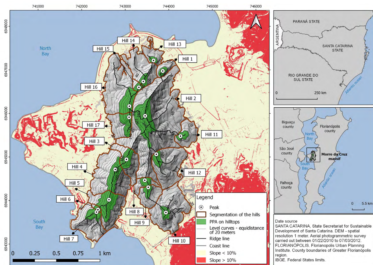
Figure 9. Hilltop PPAs in the Morro da Cruz Massif were identified using a minimum watershed size of 500 pixels, in accordance with the criteria outlined in the repealed Forest Code and Conama Resolution 303/2002.
