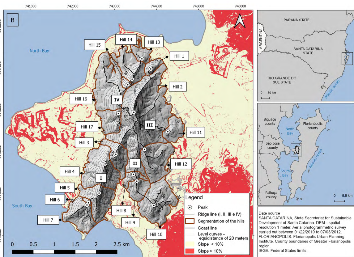
Figure 6. Relief features in the Morro da Cruz massif with minimum watersheds sizes of 15,000 pixels (A) and 500 pixels (B).
