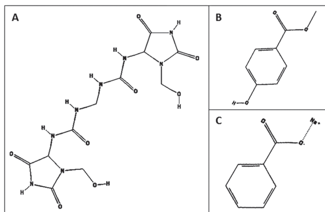
FIGURE 1 - Chemical structures of studied compounds. (A) Imidazolidinyl urea, (B) methylparaben, and (C) sodium benzoate. Source , PubChem (2005a,b,c).
