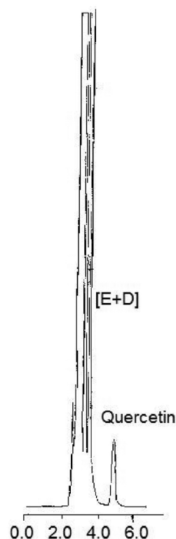
FIGURE 1 – Chromatogram of [E+D] homogenates compared to the profile of a 5 μg/mL quercetin solution. Chromatographic conditions: C18 Hypersyl BDS-CPS ciano (5 μm), 250 × 4.6 mm column - attached to a pre column, mobile phase: methanol: water (60:40 v/v) containing 2% acetic acid, 1 mL/min. Detection at 254 nm.
